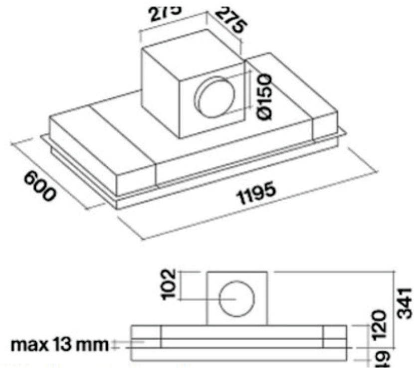
Hood and motor dimensions
